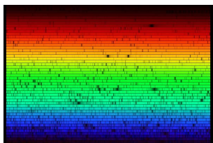
Solar Spectrum (APOD 4-23-2006)
